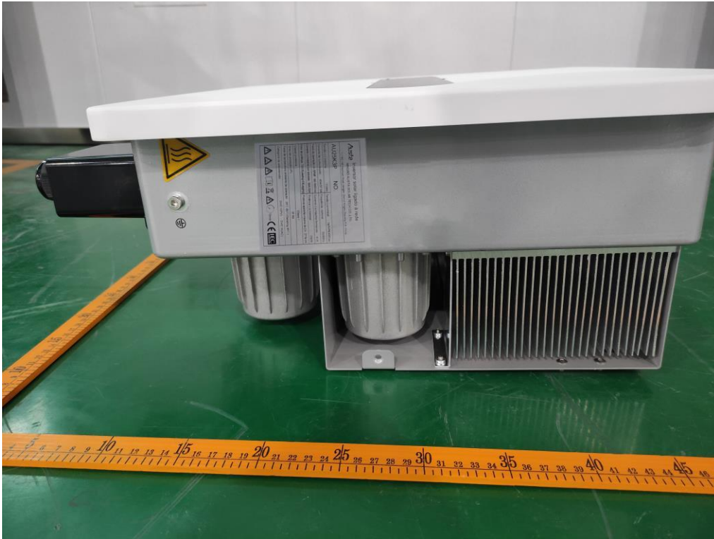
Invólucro - Vista Lateral Enclosure – Side View
