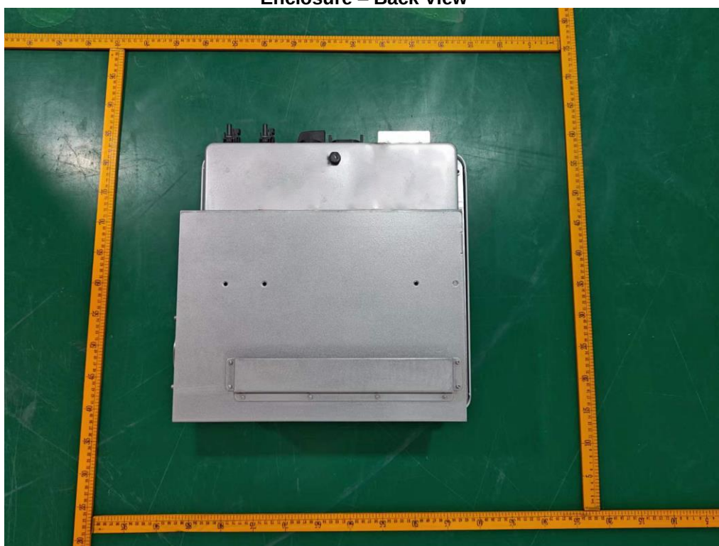
Invólucro - Vista Traseira Enclosure – Back View
