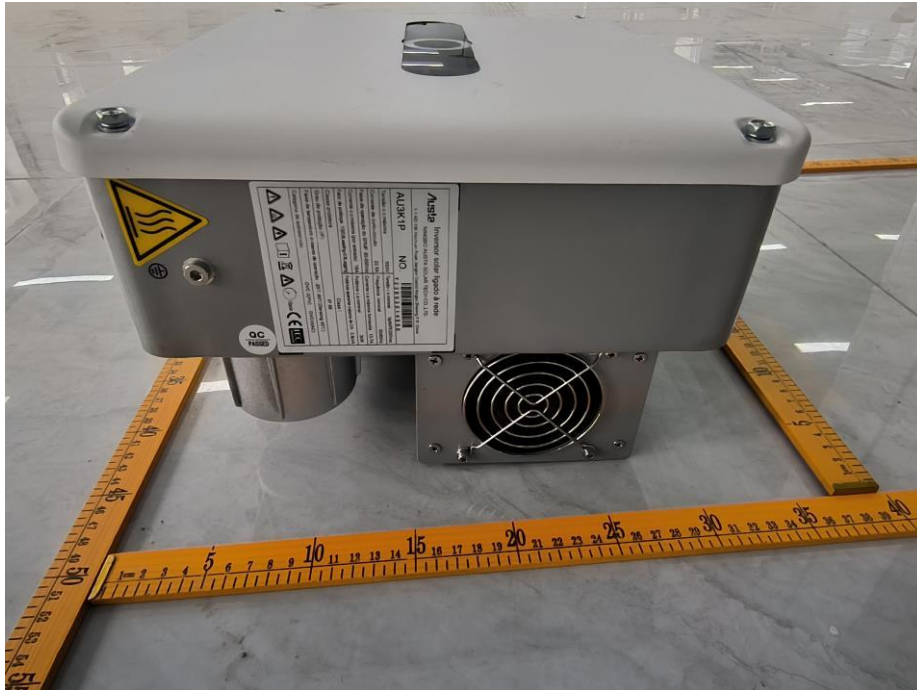
Invólucro - Vista Lateral Enclosure – Side View
